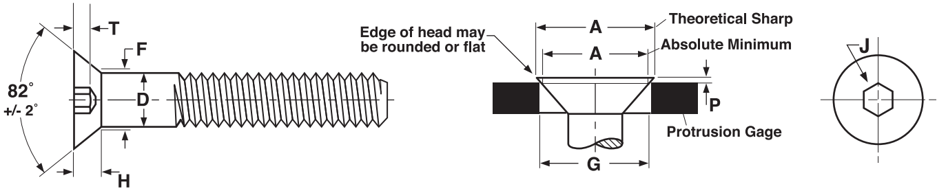
SOCKET FLAT HEAD CAP SCREWS - ALLOY STEEL ASME B18.3-2003, Blue Devil®
